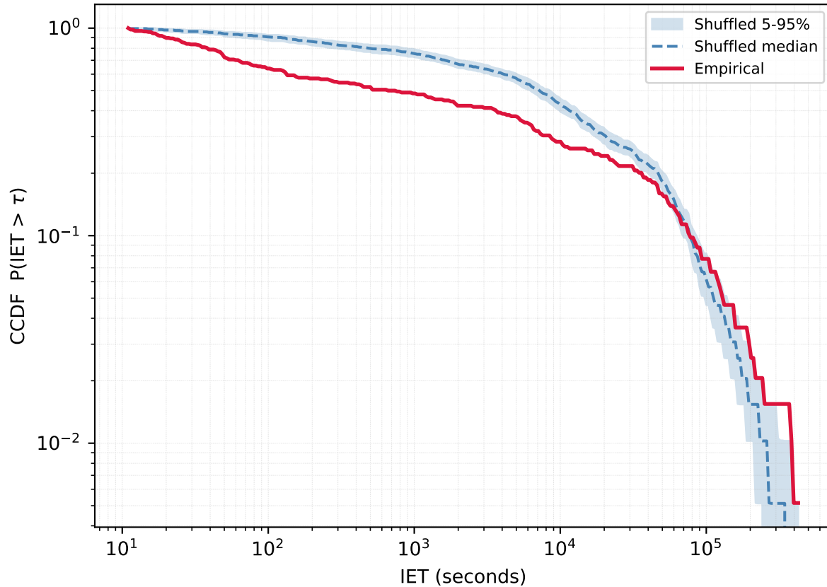
User 940028943 - Empirical vs Reshuffled | KS=0.304 p=0.000
